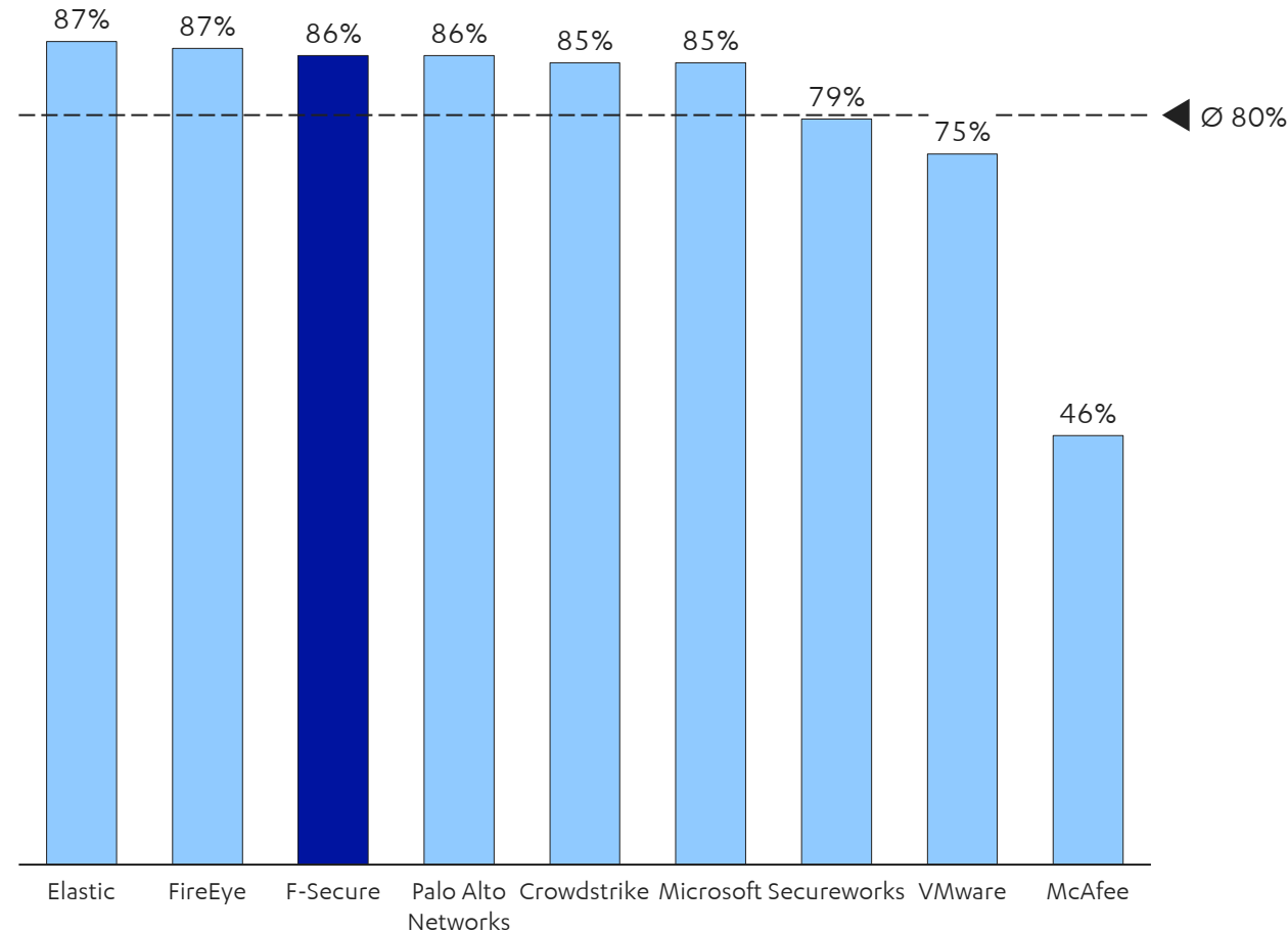
MITRE ATT&CK evaluation 2, Out-of-the-box Efficacy 2
