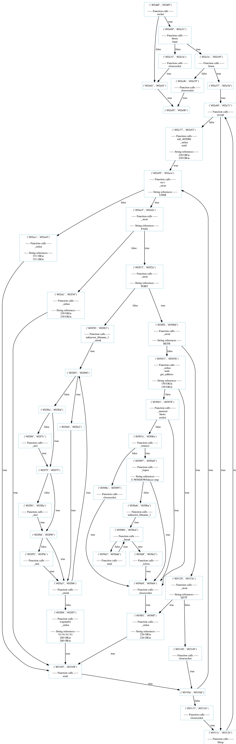
Control Flow Graph for NetSky.V FTP function
